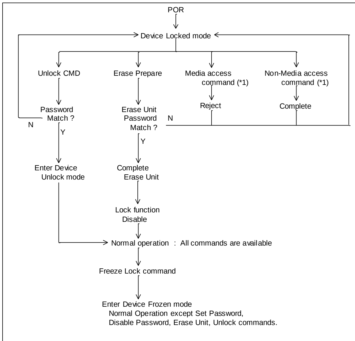
Figure 10 Usual Operation
