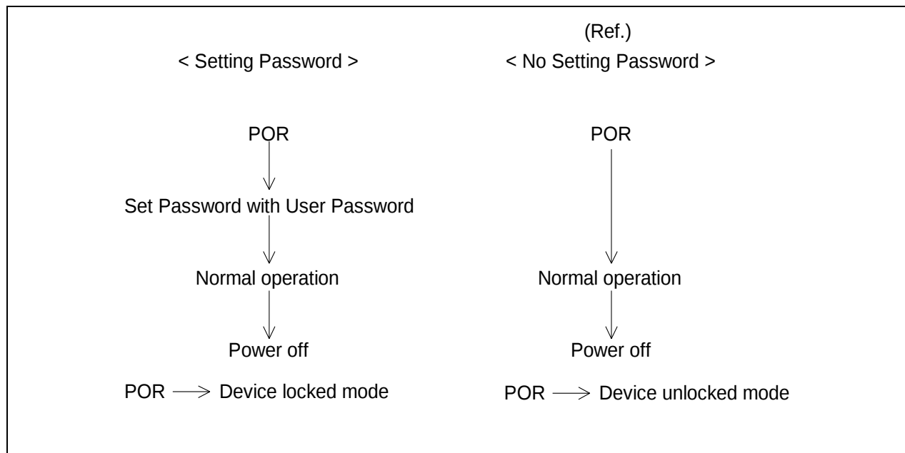
Figure 9 Initial Setting
