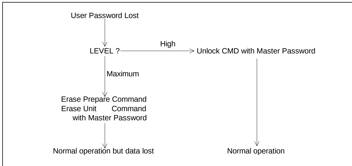
Figure 11 Password Lost
