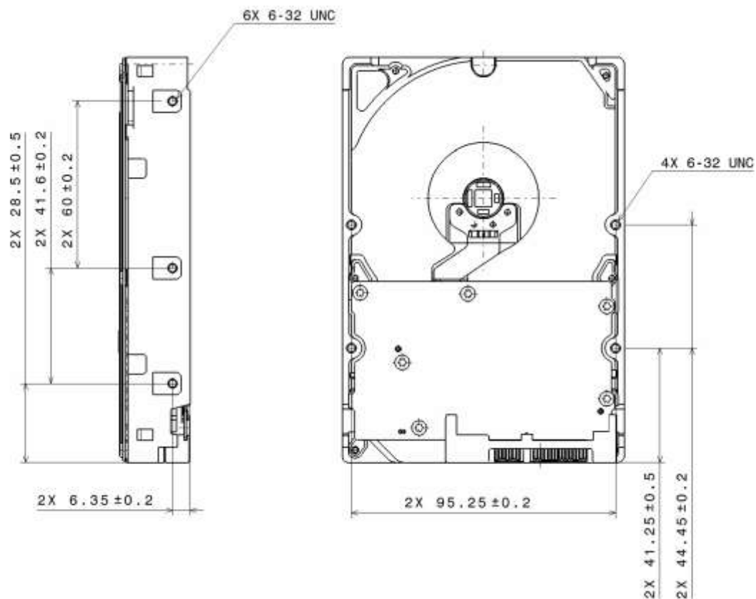
Figure 6 Bottom and side views with mounting hole locations
